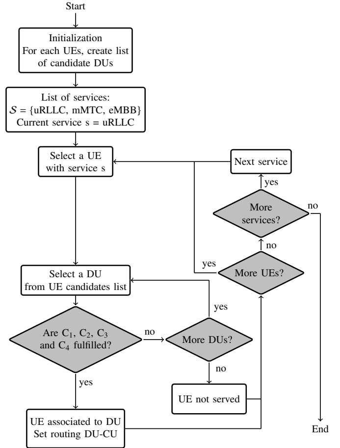
Fig. 3. Flowchart of the algorithm to allocate UEs and create slices.
