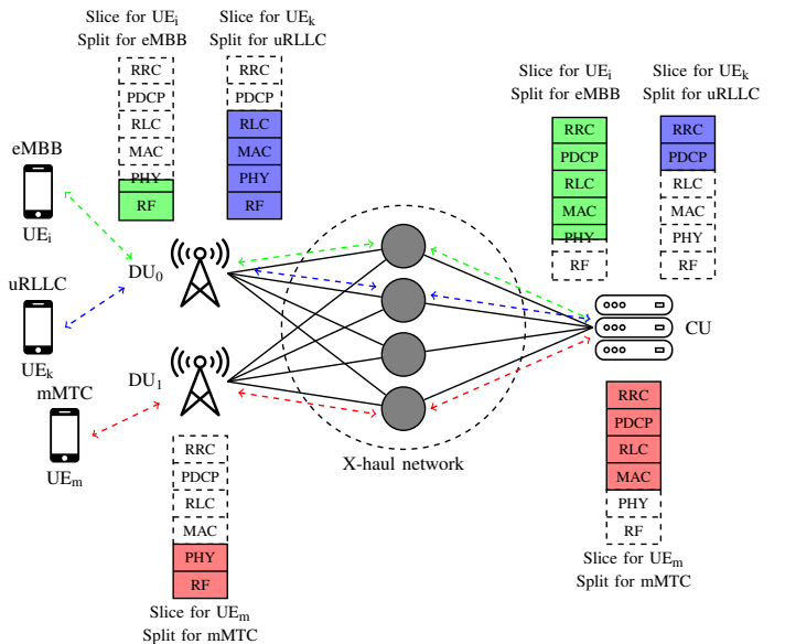
Fig. 1. Example of joint slicing and functional splitting. Each colour denotes a slice. Protocol layers are coloured where implemented.
