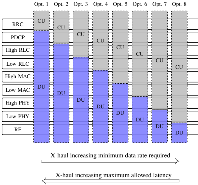
Fig. 2. Functional splits/options defined by 3GPP and allocation of protocol stack layers in the DU and CU.
