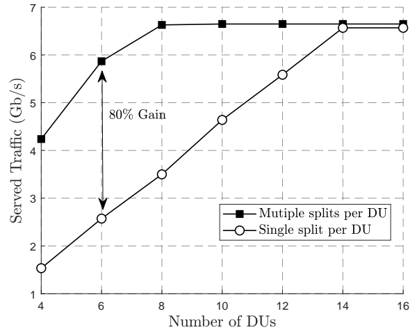
Fig. 4. Served traffic for 4 to 16 DUs. The offered traffic is 6.65 Gb/s and the capacity of the X-haul links is \infty . Results have 95% confidence level.
